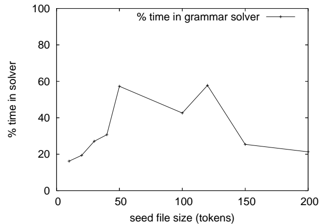
Figure 10. Grammar solver performance. The % time in solver line indicates what percentage of total 2-hour run time was spent in the grammar constraint solver.
