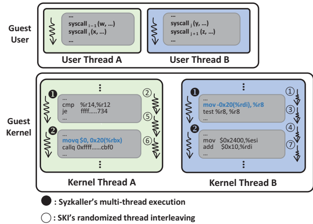
Fig. 2: Race detection mechanisms of Syzkaller and SKI
